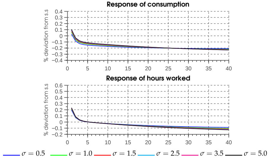
Figure 4: Preferences à la Greenwood, Hercowitz, and Huffman (1988) with changing \sigma
