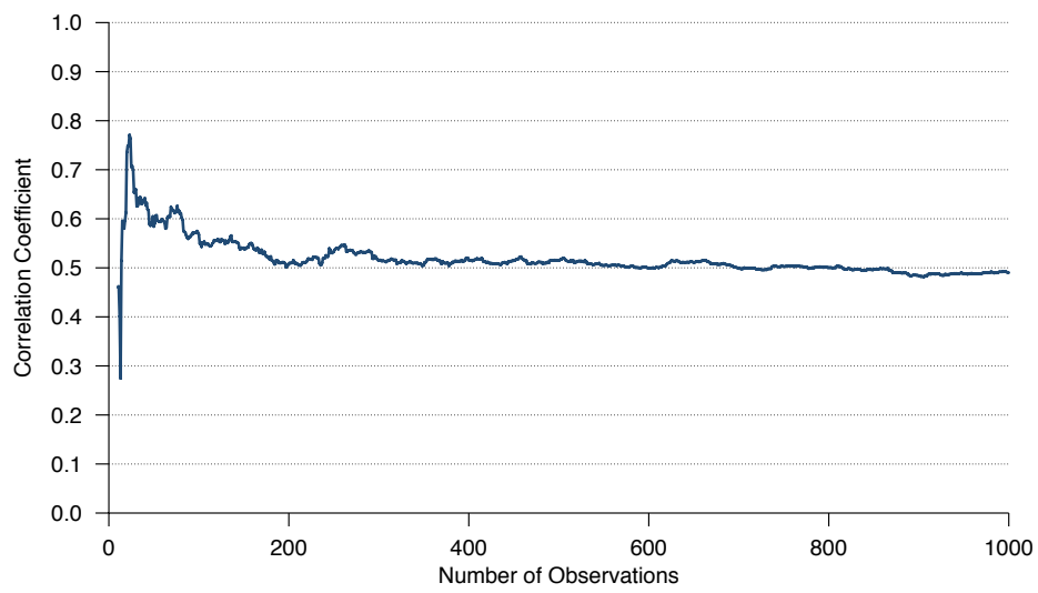
Figure 6: Rolling Correlation Coefficient
